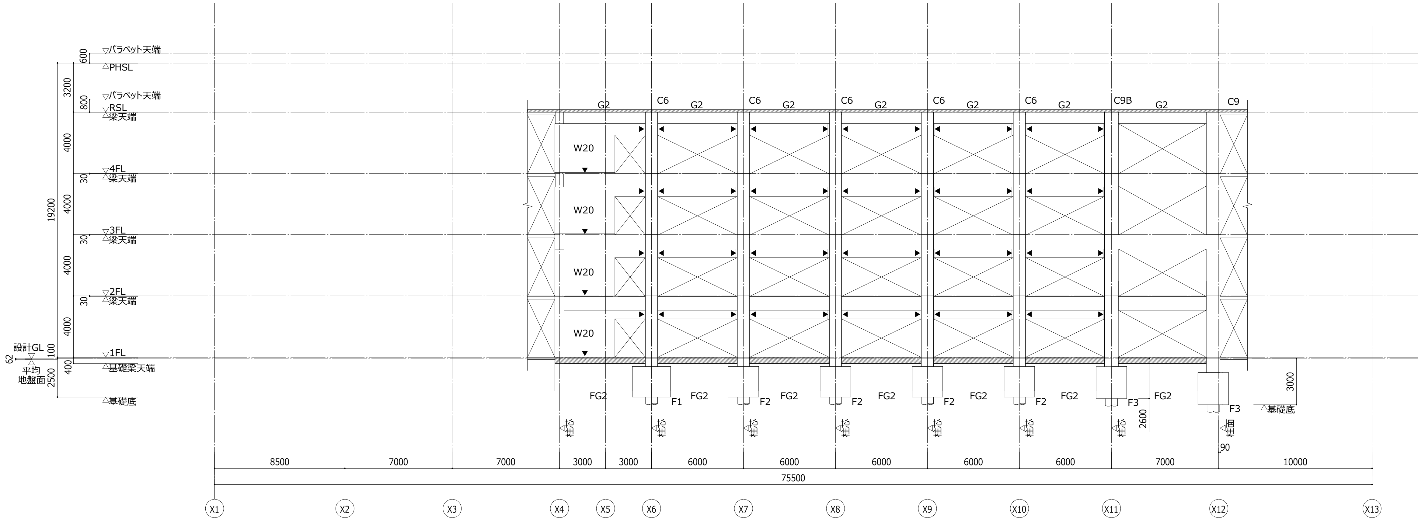
Y13 通り軸組図 1/150 [A1] 1/300 [A3]
