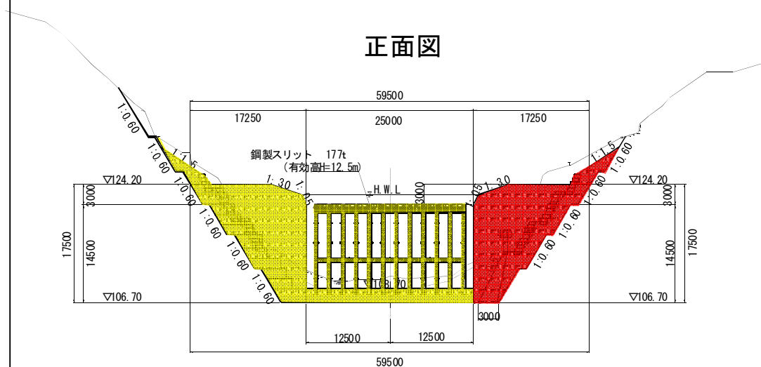
①砂防えん堤工 (H=14.5m, L=59.5m)
