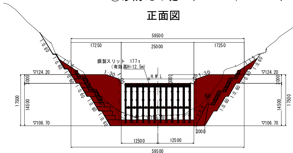
①砂防えん堤工 (H=14.5m, L=59.5m)
