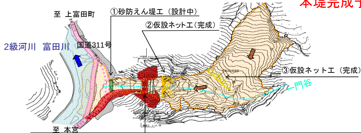
①砂防えん堤工 (H=14.5m, L=59.5m)
