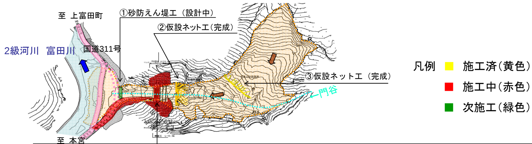
①砂防えん堤工 (H=14.5m, L=59.5m)
